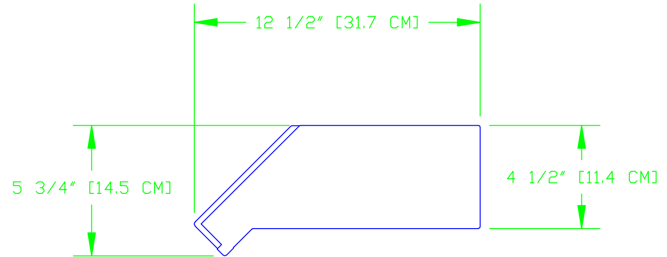
SIDE VIEW
