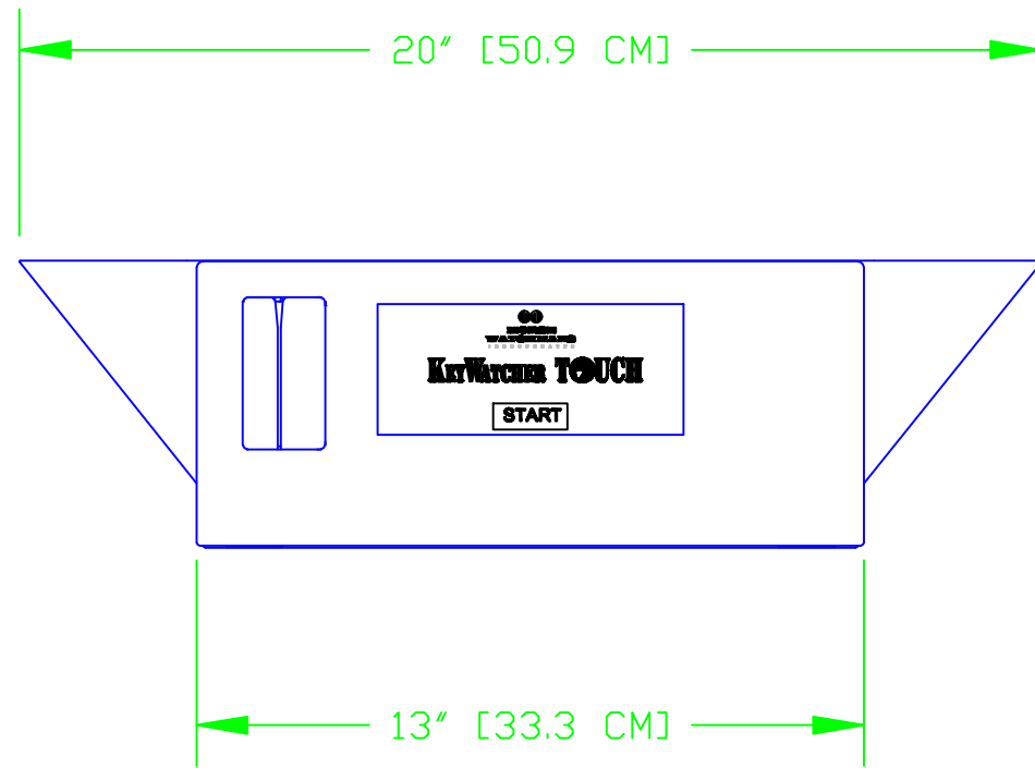
FRONT VIEW
