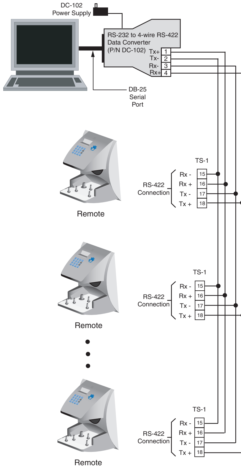
Figure 7-7: Host PC Network System Wiring Diagram
